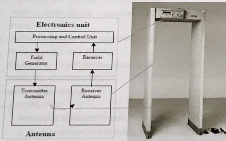
Gambar 1. Contoh peralatan Walkthrough Metal Detector
